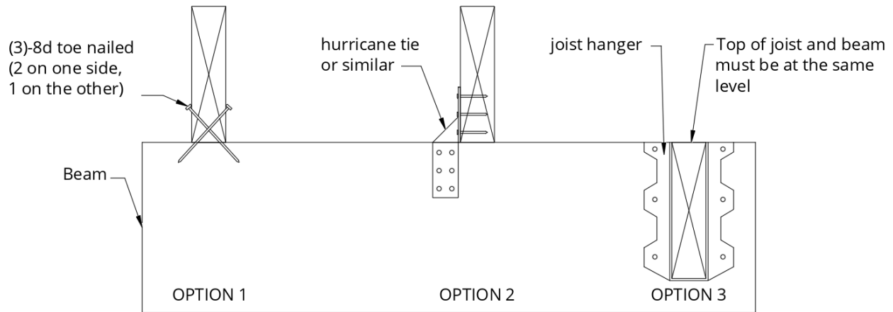
FIGURE 17 - JOIST ATTACHMENT
