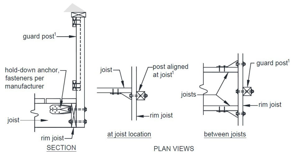
Figure 30 - Guardrail Post Connection Detail
