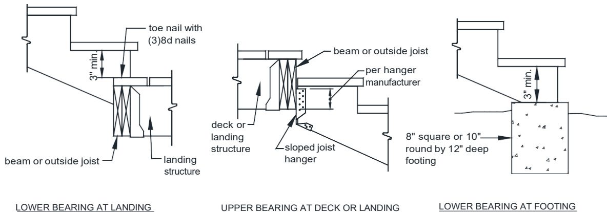
FIGURE 32 - STRINGER BEARING
