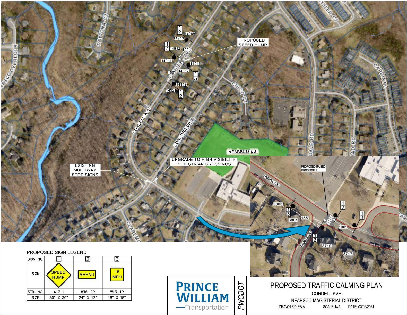
Figure: Cordell Avenue Traffic calming plan
