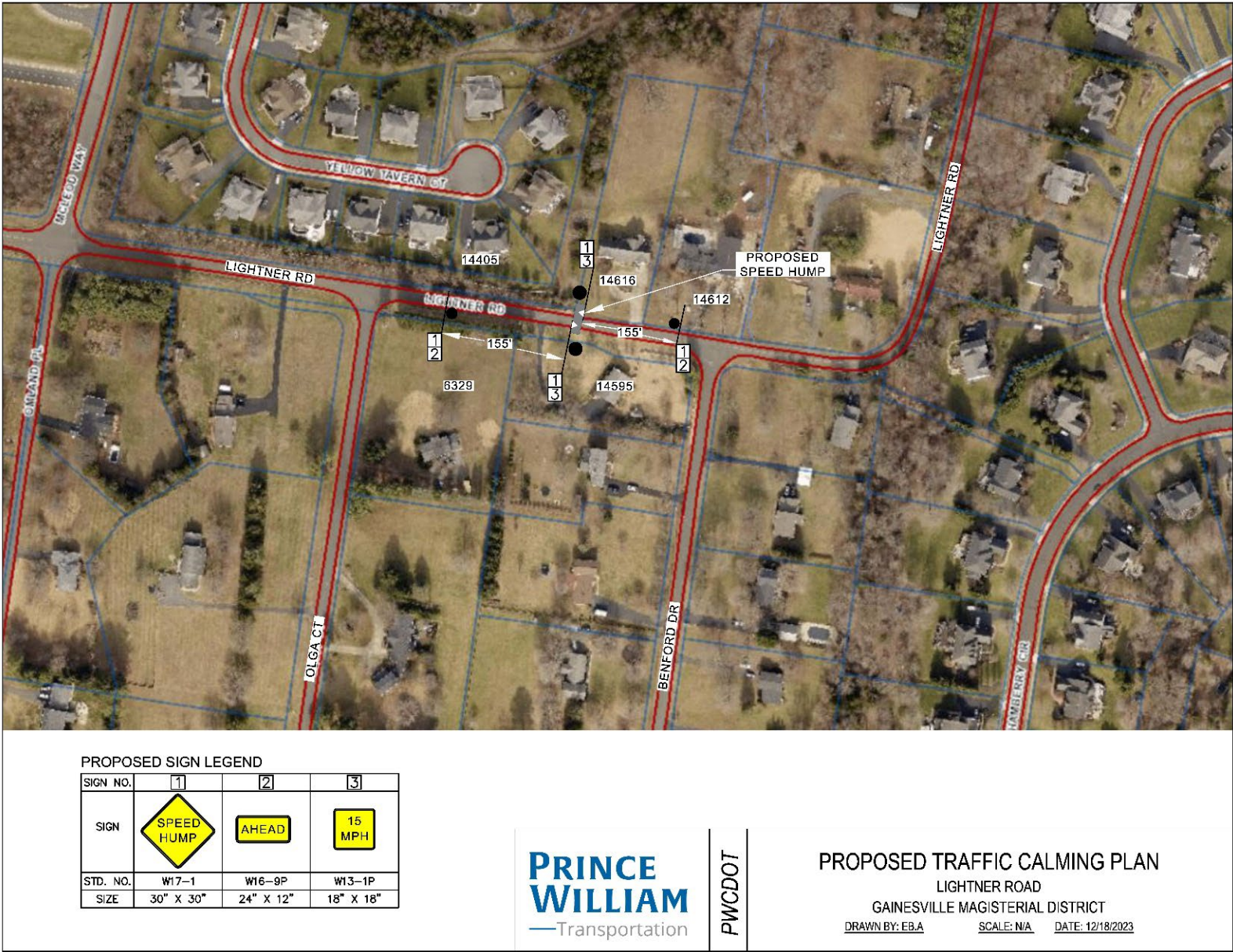
Figure: Lightner Road Traffic calming plan
