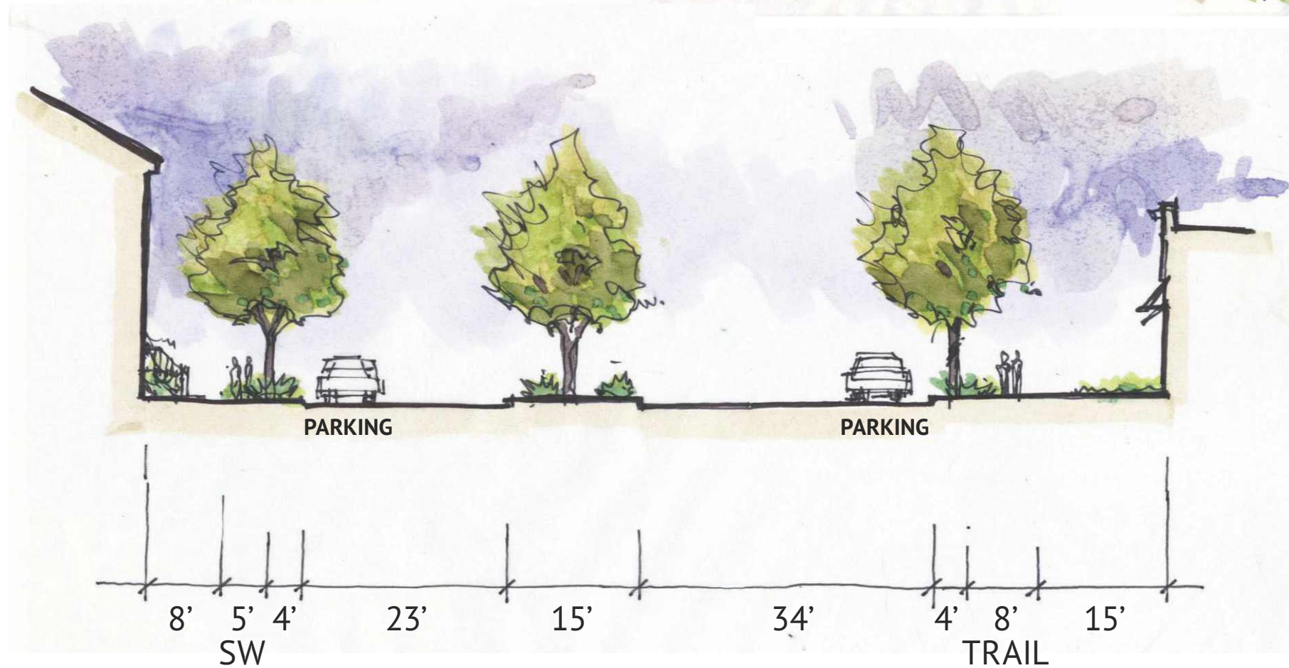
Streetscape Section Approximate Scale: 1/16"=1'-0"
